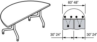
Half Moon Table - Spider Legs
