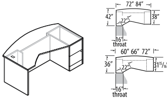
Single Pedestal Bow Top Extended Corner Desk - RIGHT
