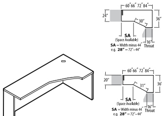
Right Extended Corner, 16" Throat
