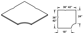
Bi-Functional 90° Corner Worksurface
